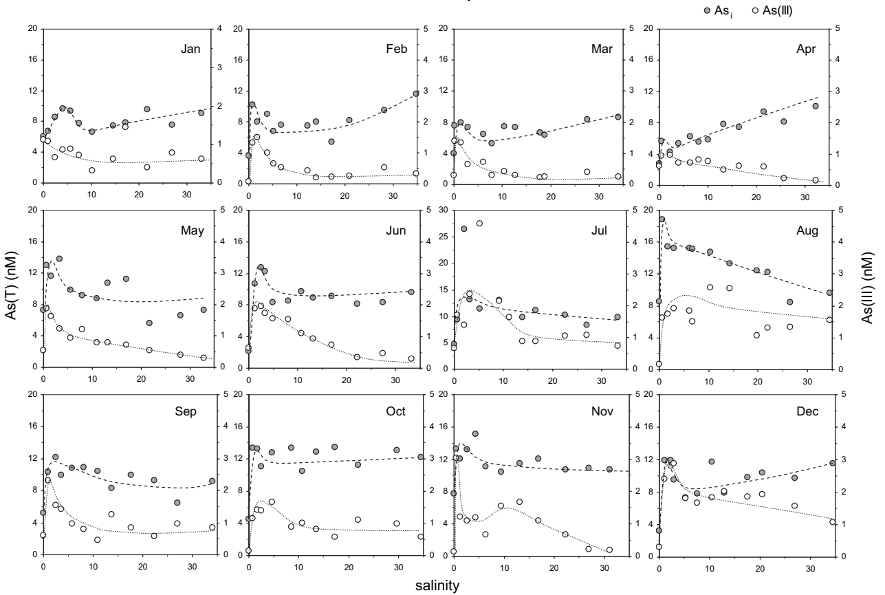
Fig. 4. (a) POC, PO 4 3- , chl-a-to-phaeopigments and E/SHE, (b) As I and As(III), (c) PAs and PPb salinity distributions over the seasonal cycle.
