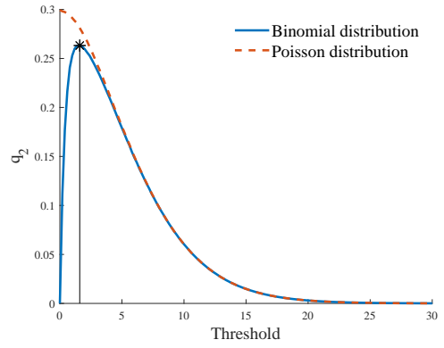
Fig. 1. q_2 with both Poisson and binomial laws, \gamma = 2
