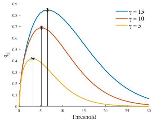
Fig. 2. q_2 with respect to threshold for different values of \gamma
