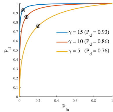
Fig. 3. ROC curves for different values of \gamma
